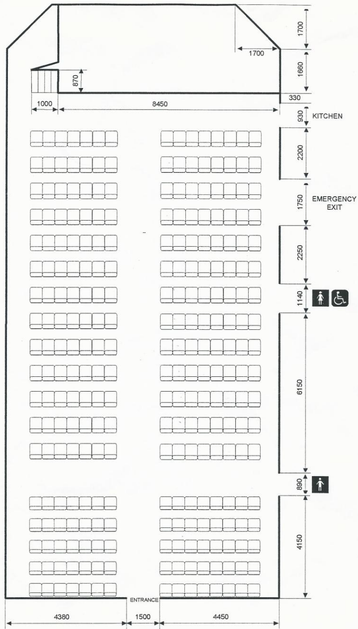
Victoria Hall, Ellon Floorplan - 270 Seat Layout
